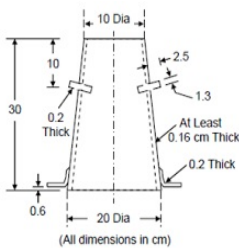
Fig. 1: Schematic Slump Cone Apparatus
