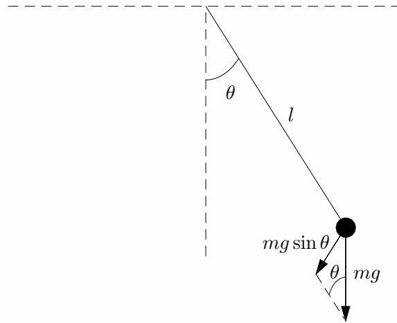
Figure 3.3: The pendulum.
