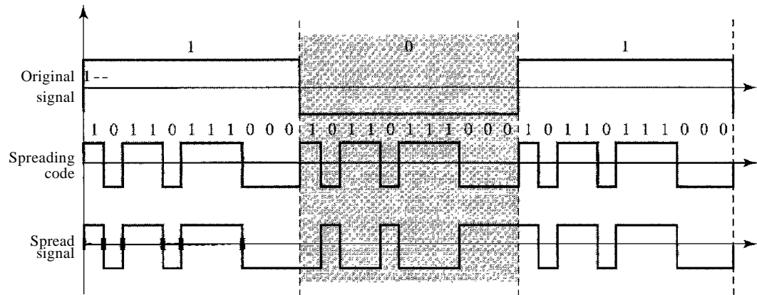
Figure 6.33 DSSS example
