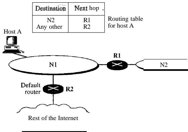
Figure 22.4 Default method
