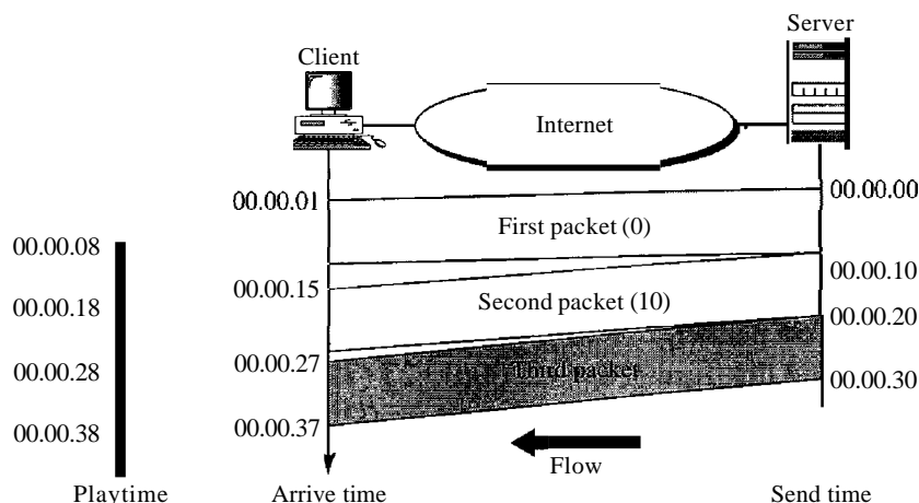
Figure 29.16 Timestamp
