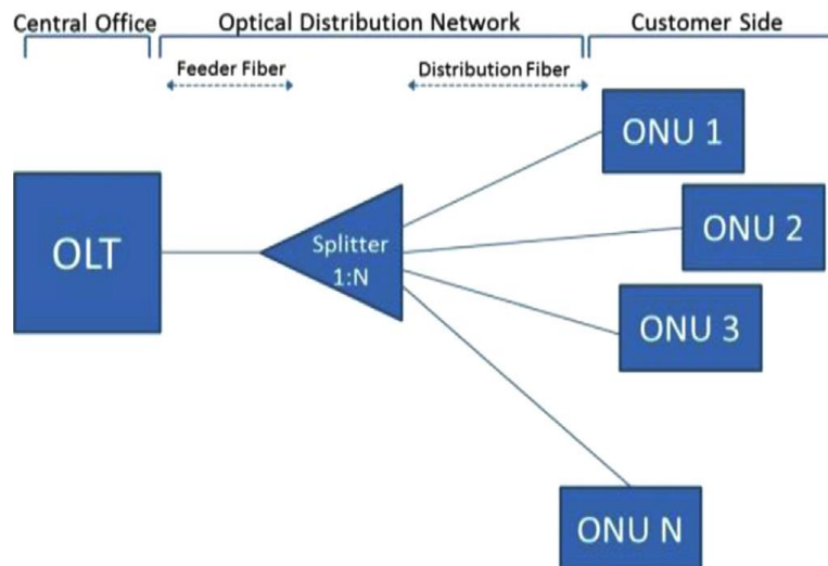
Fig. 1. PON architecture.
