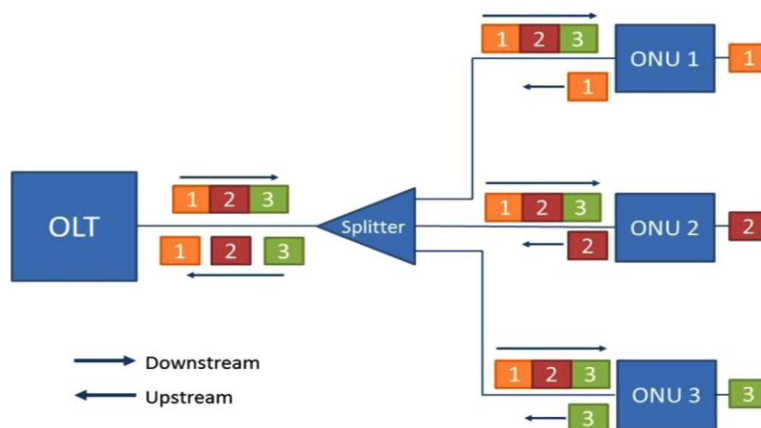
FIG 1 TDM Architecture
