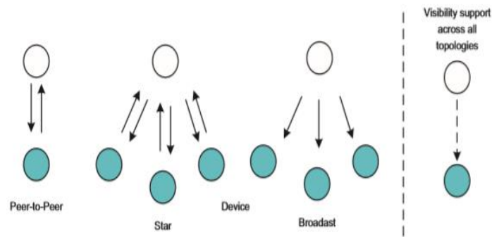
Fig. 10. Supported MAC topologies by IEEE 802.15.7 [25].
