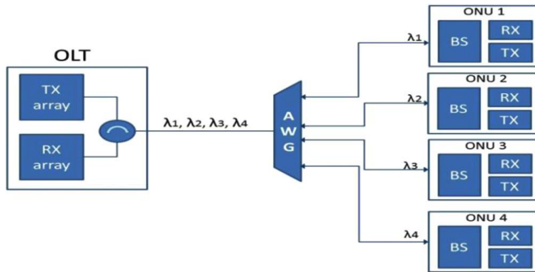
Fig 2 WDM PON
