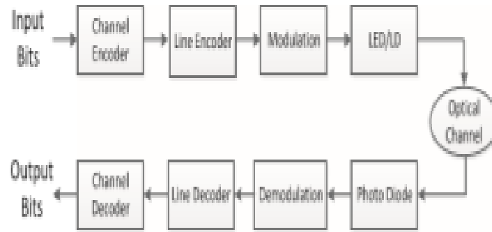
Fig. 12. Typical physical layer system model of VLC.
