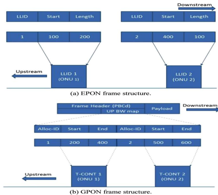
Fig. 3. Frame structure (a) EPON, (b) GPON.
