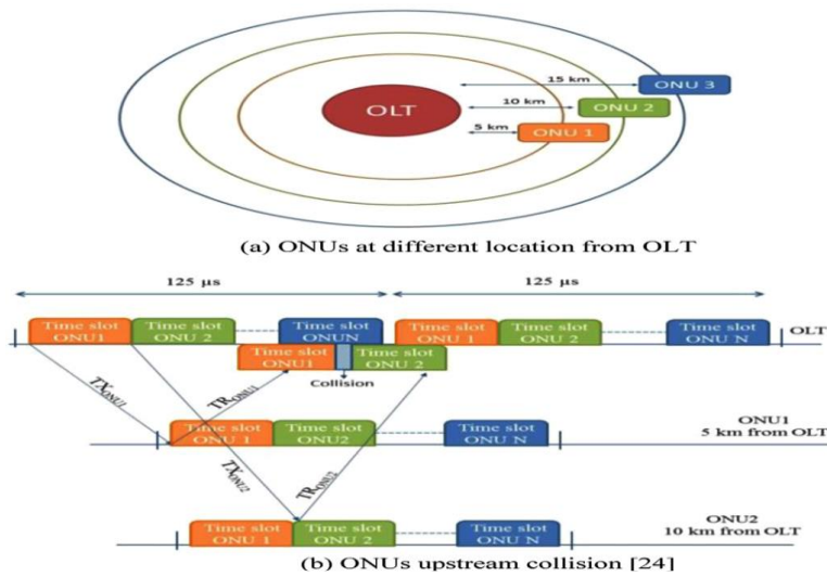
Fig. 4. (a) ONUs at different location from OLT. (b) ONU sup stream collision (Kra-mer,1999).
