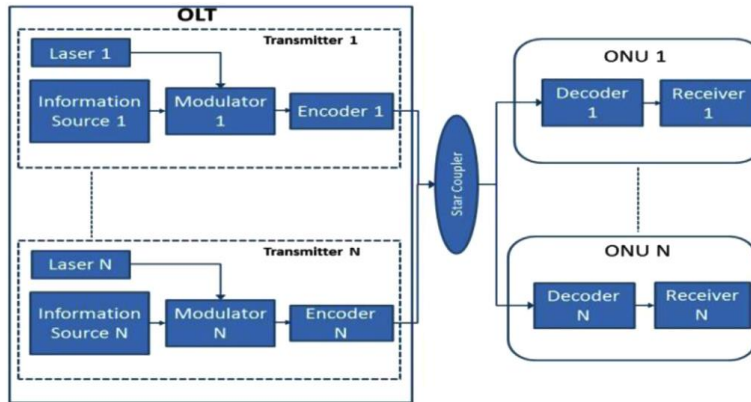
Fig 3 OCDFM Architecture
