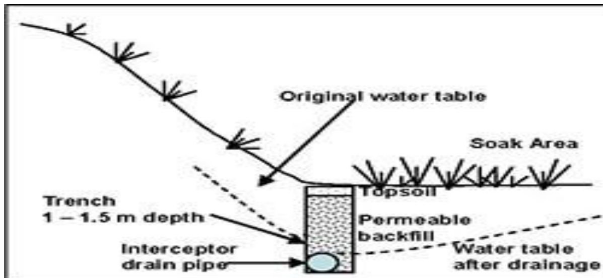
Subsurface drainage (diagram)
