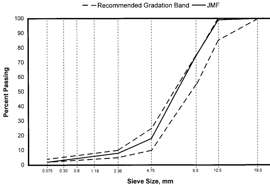
Figure 6. Gradation of OGFC Field Test Sections.
