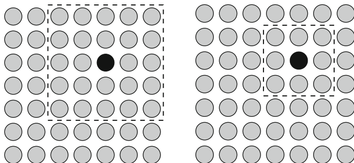
Fig. 14.7 The idea of “neighborhood” in the Kohonen network
