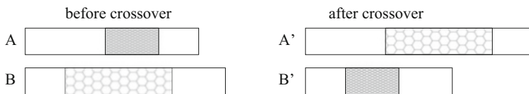
Fig. 16.7 The two-point crossover operator creates the children by exchanging randomly selected substrings in the parent chromosomes
