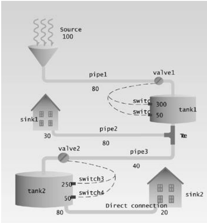
Figure 13.6 A typical water system.
