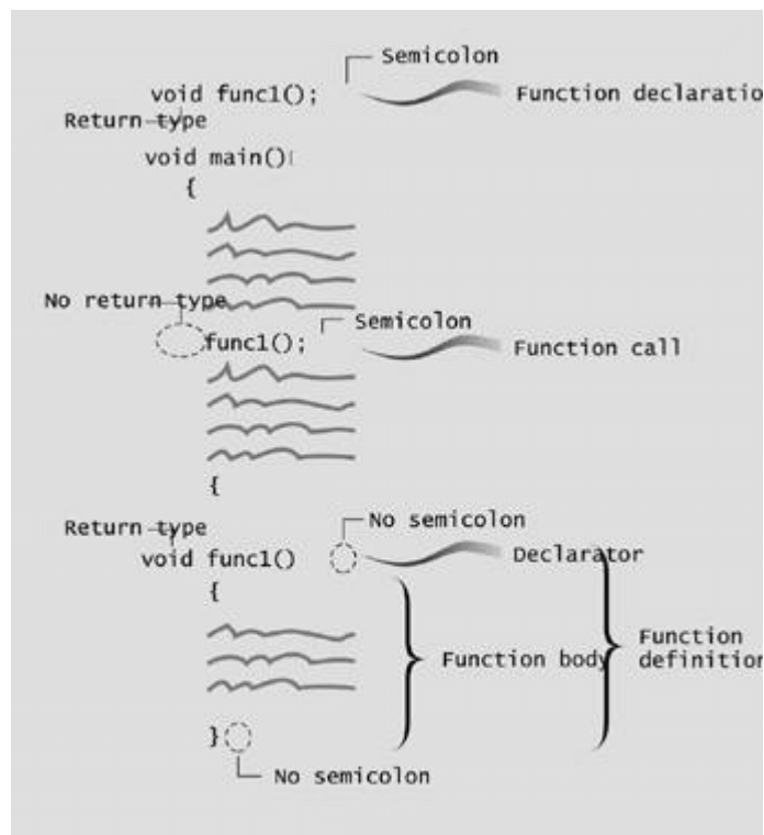
Figure 5.2 Function syntax.
