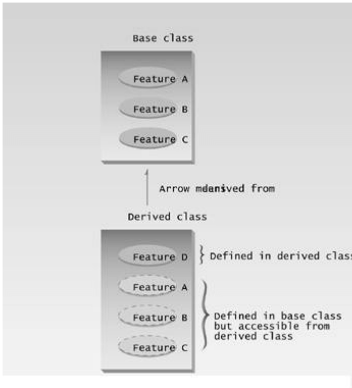
Figure 9.1 Inheritance.
