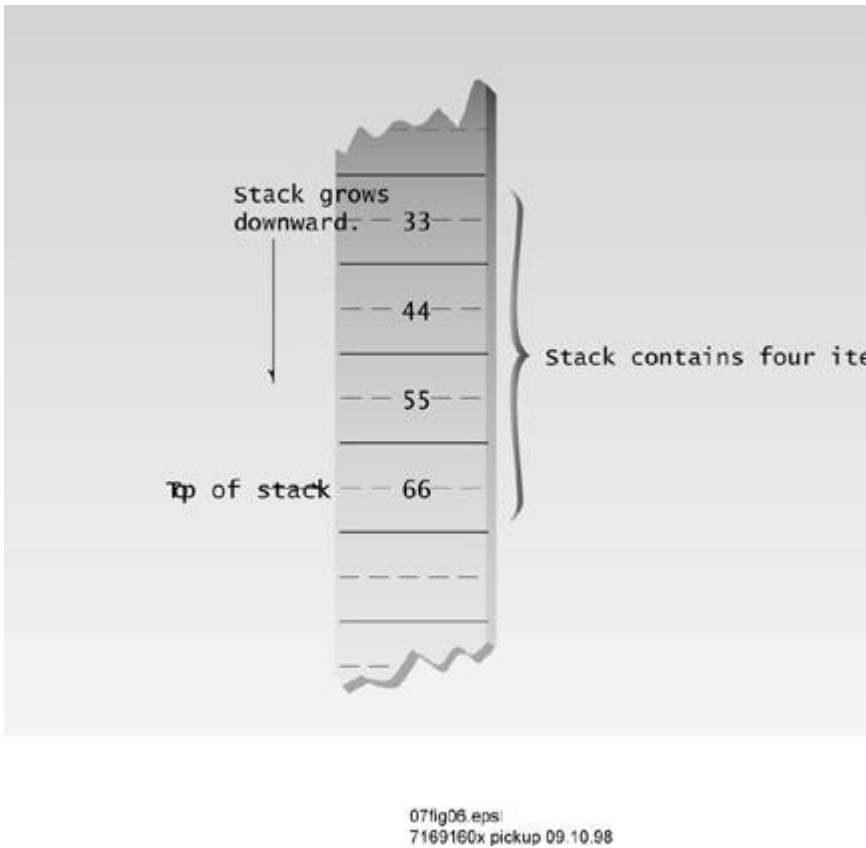
Figure 7.6 A stack.
