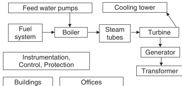
Fig. 9.3 Power station block diagram
