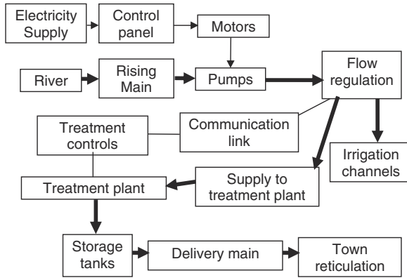
Fig. 15.6 Flow chart for water supply system
