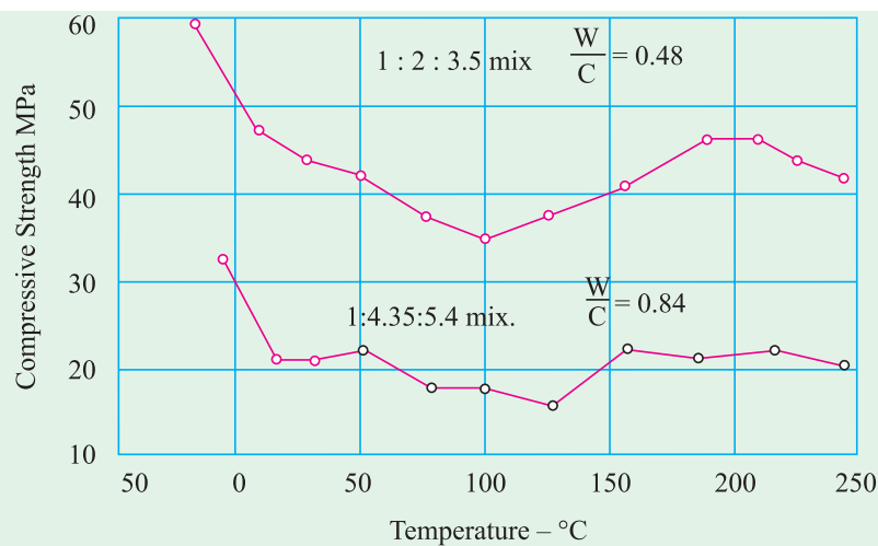
Fig. 9.16. Compressive strength of concrete after heating to different temperatures
