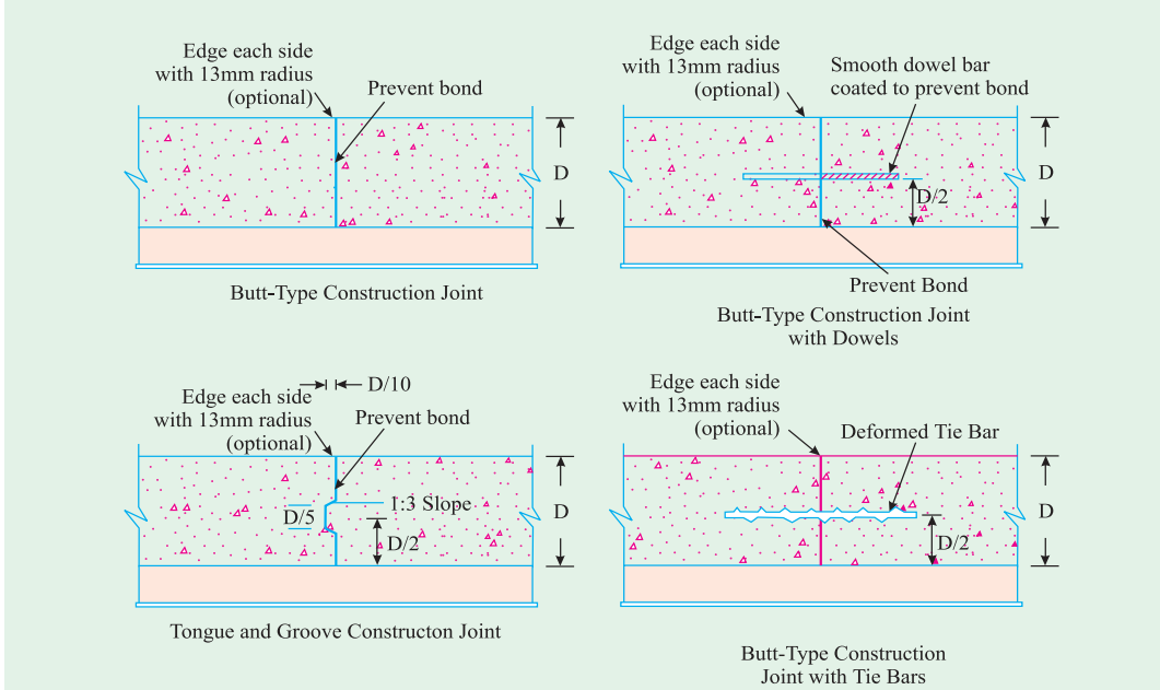
Fig. 9.10. Construction Joints
