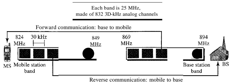
Figure 16.3 Cellular bands for AMPS
