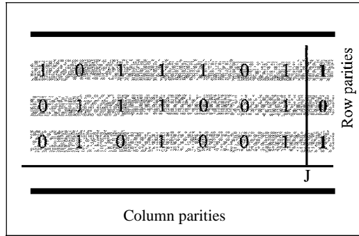
Figure 10.11 Two-dimensional parity-check code
