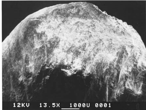
Fig. 14.17 SEM micrograph of jagged surface and striations on deer antler beam, produced by its use as a soft-hammer percussor for stone artifact production by Sandra L. Olsen (1989:132, Fig. 7). Scale: bar is 1000 microns. Compare with Fig. 13.13 for natural antler modification image. (Used with permission of S. L. Olsen and Elsevier)
