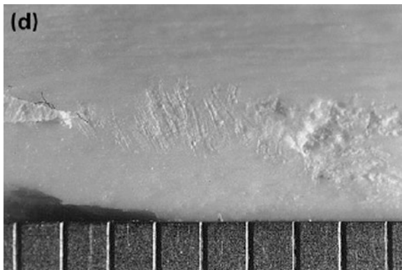
Fig. 14.14 Experimentally produced stone anvil percussion pits (right) and striae field (center) on a bovid long bone, at c. 16x magnification (Photo from Blumenschine et al. (1996:498, Fig. 2d), used with permission of Elsevier)
