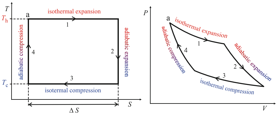
Fig. 5.2 The T - S and P - V diagram for the working fluid in a Carnot heat engine cycle. The four steps of the cycle are denoted by subsequent numbers starting from state a. A Carnot refrigerator or heat pump operates on the same cycle but in the reverse direction; its steps follow each other as 4 - 3 - 2 - 1
