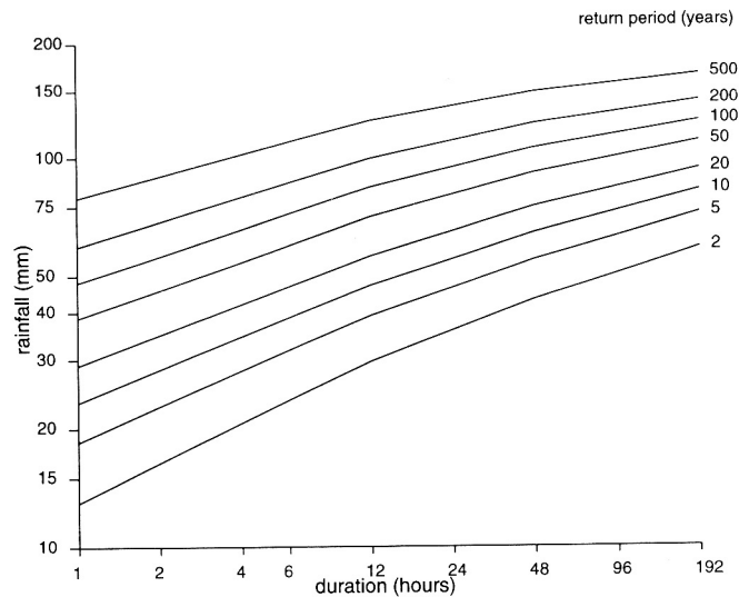
Figure 5 Depth-Duration-Frequency curves
