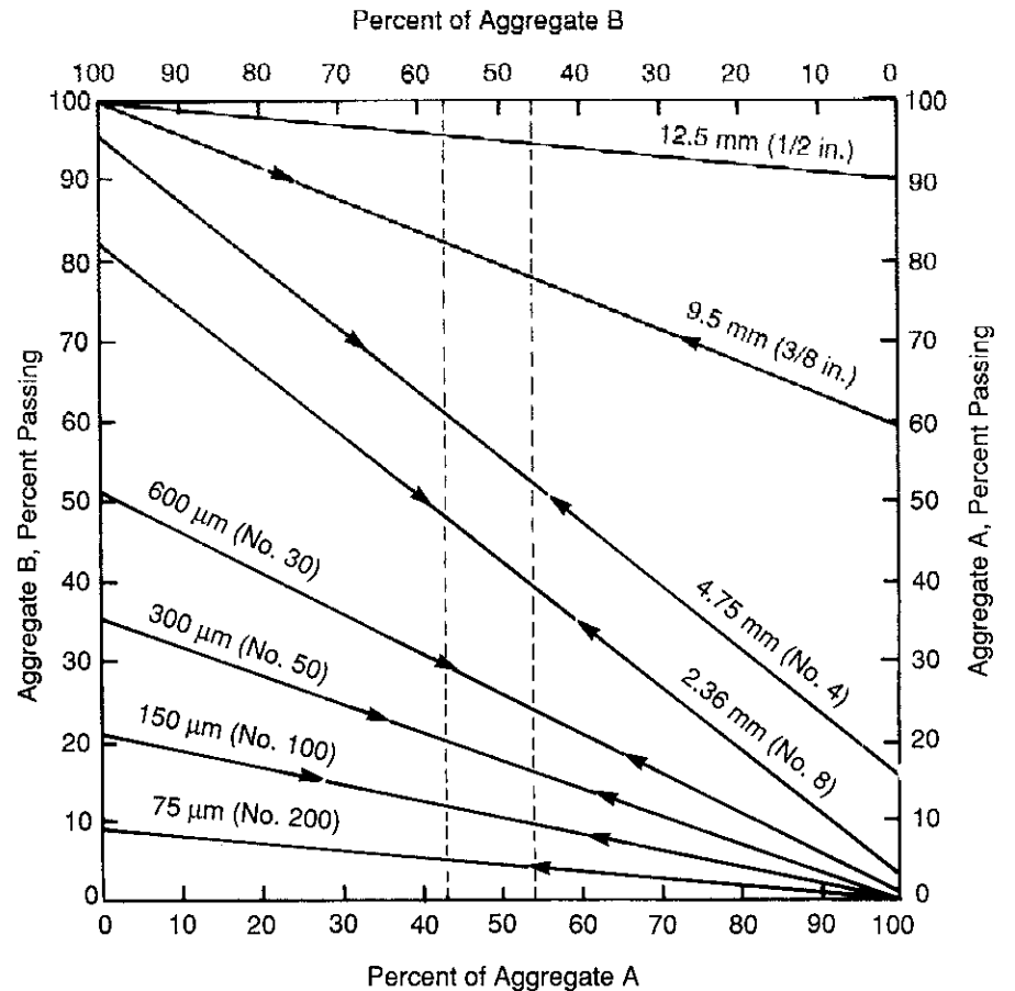
Figure 3.4 – Graphical solution for proportioning two aggregates
