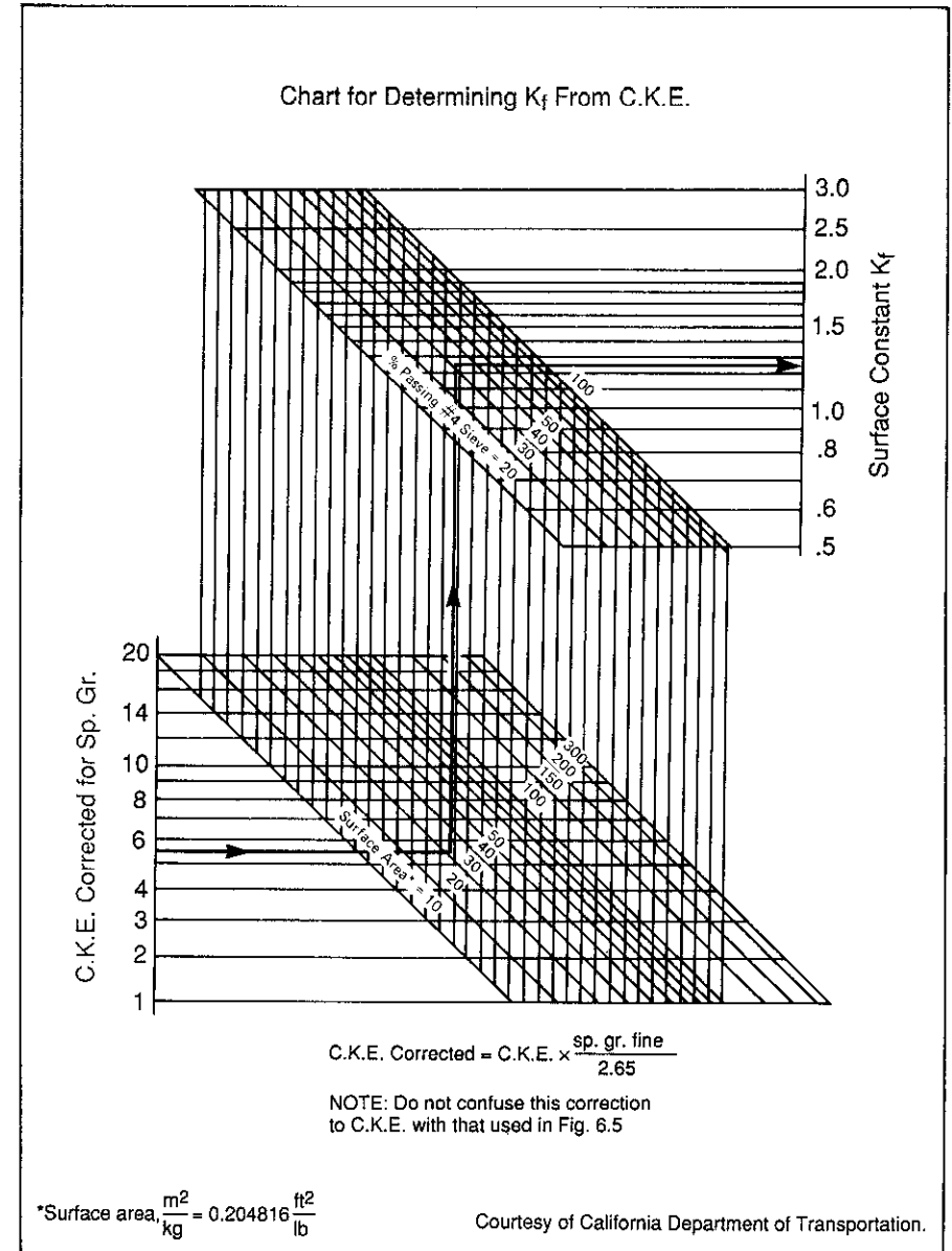
Figure 6.2 – Chart for determining surface constant for fine material, K f from C.K.E., Hveem method of design
