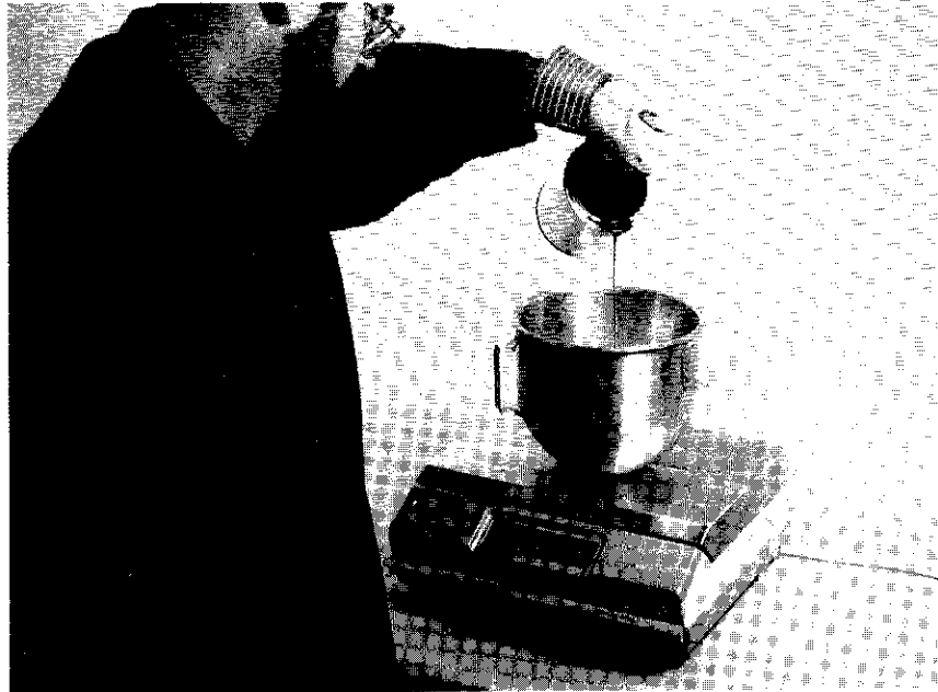
Figure 2.8 – Adding asphalt to heated aggregate
