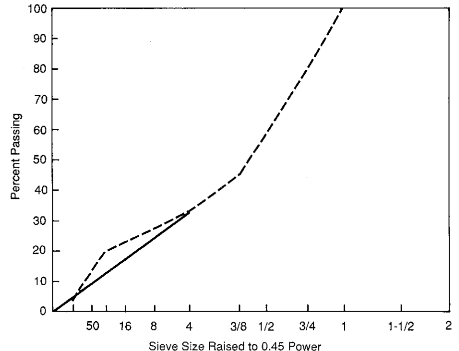
Figure 3.7 – Example of a "humped" gradation
