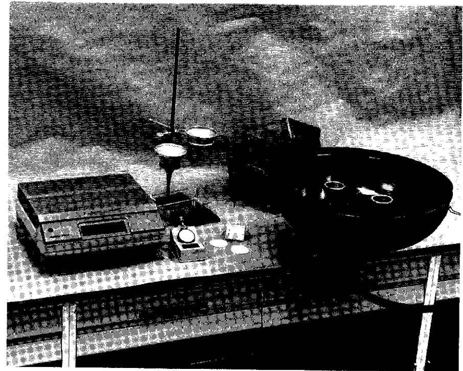
Figure 6.1 – Apparatus for Hveem C.K.E. tests
