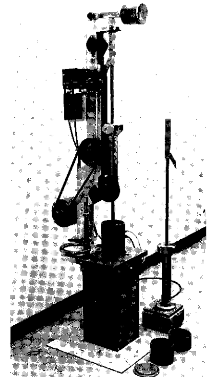
Figure 5.1 — Pedestal, hammer (mechanical) and mold used in preparing Marshall test specimens
