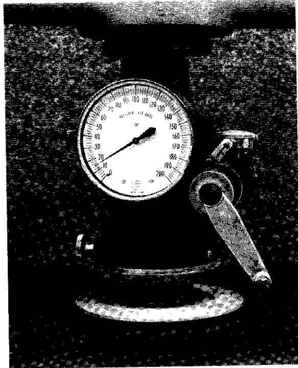
Figure 6.13 – Hveem stabilometer
