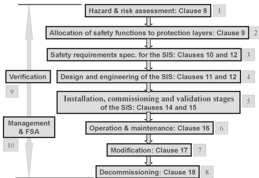
Figure 7. 8 IEC 61511-safety lifecycle model
