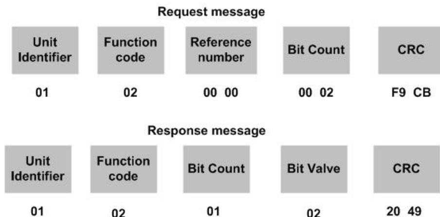
Figure 5.9 Example: FC02-reading input discretés
